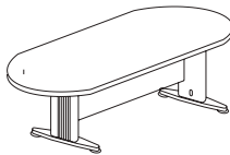
OVAL CONFERENCE TABLE TO 18 1800W x 900D x 745H TO 24 2400W x 1200D x 745H
