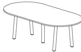
OVAL CONFERENCE TABLE BO 18 1800W x 900D x 750H (4 BWL 725 + 1 BW 725) BO 24 2400W x 1200D x 750H (6pcs of BWL 725)
