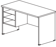
EXS 1060 SIDE TABLE 900W x 450D x 700H
