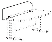
CURVE PARTITION BOARD With PARTITION BRACKET TPO 1200 1200W x 400D x T16 TPO 1500 1500W x 400D x T16 TPO 1800 1800W x 400D x T16 DarkGrey&LightGrey
