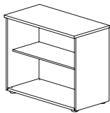
BO 825 LOW CABINET 804W x 407D x 852H
