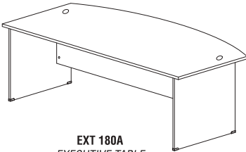
EXT 180A EXECUTIVE TABLE 1800W x 900D x 745H
