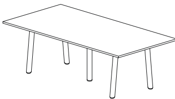
RECTANGULAR CONFERENCE TABLE BV 18 1800W x 900D x 750H (4 BWL 725 + 1 BW 725) BV 24 2400W x 1200D x 750H (6pcs of BWL 725)
