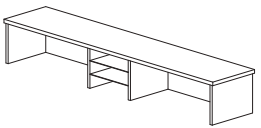
COUNTER TOP EXC 180 1800W x 300D x 300H EXC 150 1500W x 300D x 300H EXC 120 1200W x 300D x 300H
