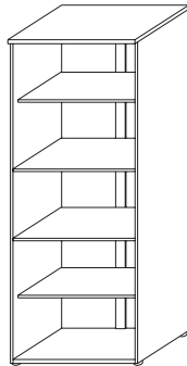
TO 2025 HIGH CABINET 800W x 405D x 2057H
