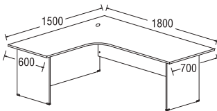
SUPERIOR COMPACT TABLE(L) EXL 552 1500W x 1500D x 600 x 600 x 745H EXL 1815 1800W x 1500D x 700 x 600 x 745H EXL 1515 1500W x 1500D x 700 x 600 x 745H
